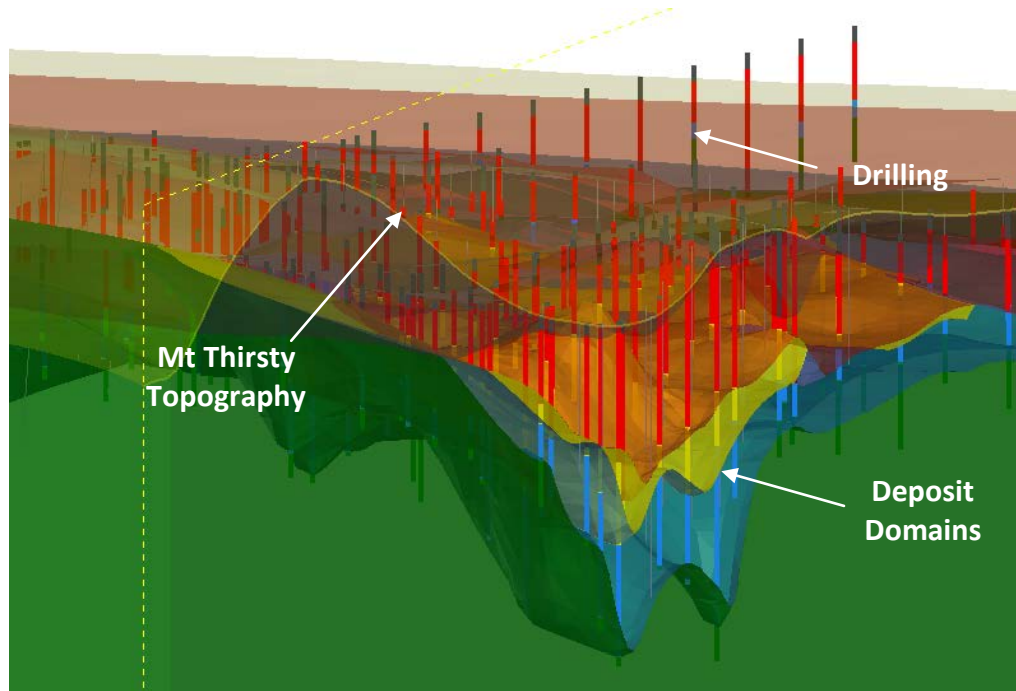
Figure 2: 3D cut away isometric of the Mt Thirsty deposit looking south west.
