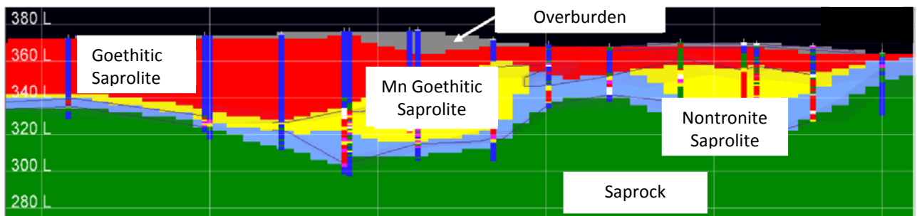
Figure 3: Geological domain model typical cross section.
