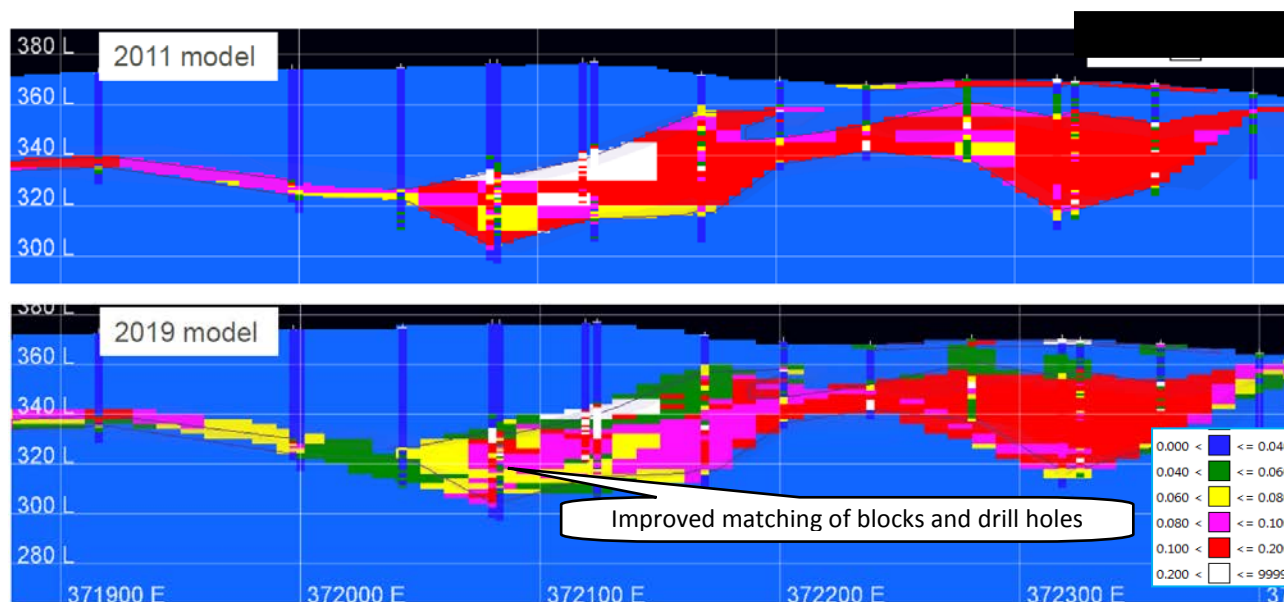
Figure 4: Comparison between 2011 and 2019 block models coloured by cobalt on section 6447600mN.
